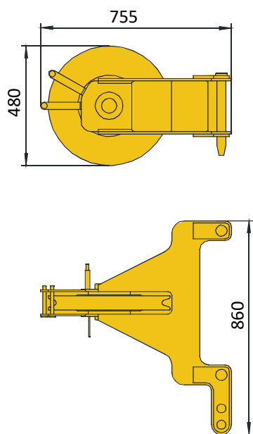
Auxiliary sheave 95kg
