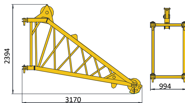
Independent jib head 453kg
